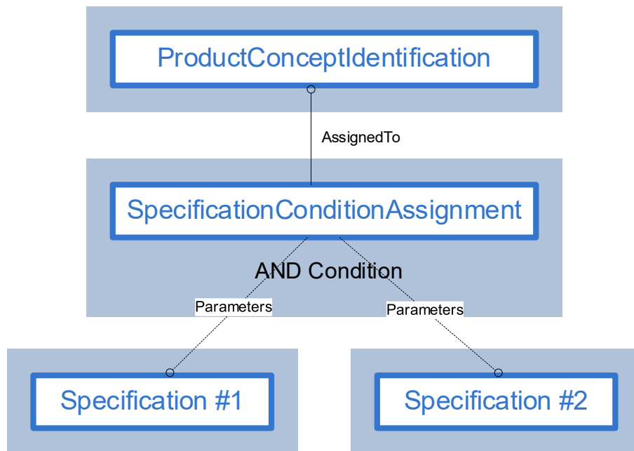
Figure 38: Example for an AND Condition for specifications
