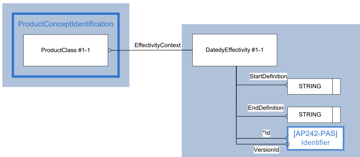
Figure 24: Instance Model Date Effectivity
